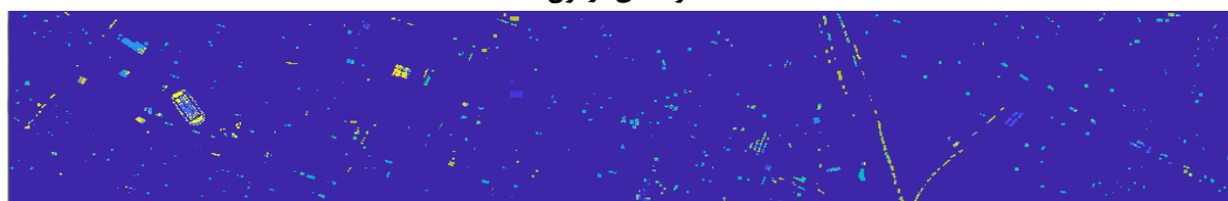
DSM-SVM
