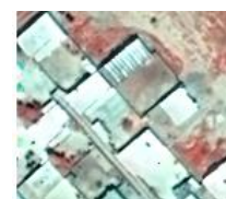
Win size = 11×11
