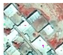
Win size = 9×9
